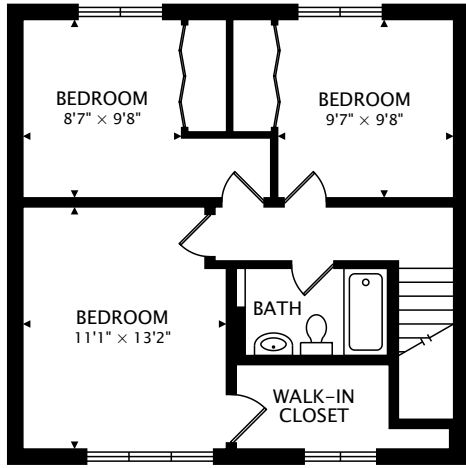
SECOND 624 sq ft
