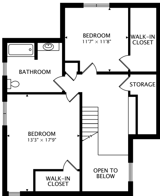
SECOND 799 sq ft
