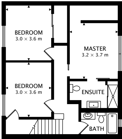
SECOND 70.7 m 2
