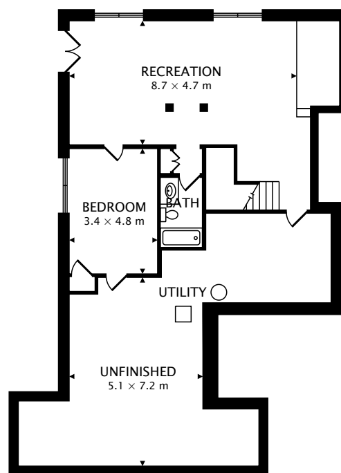
LOWER 173.5 m 2 BELOW GRADE
