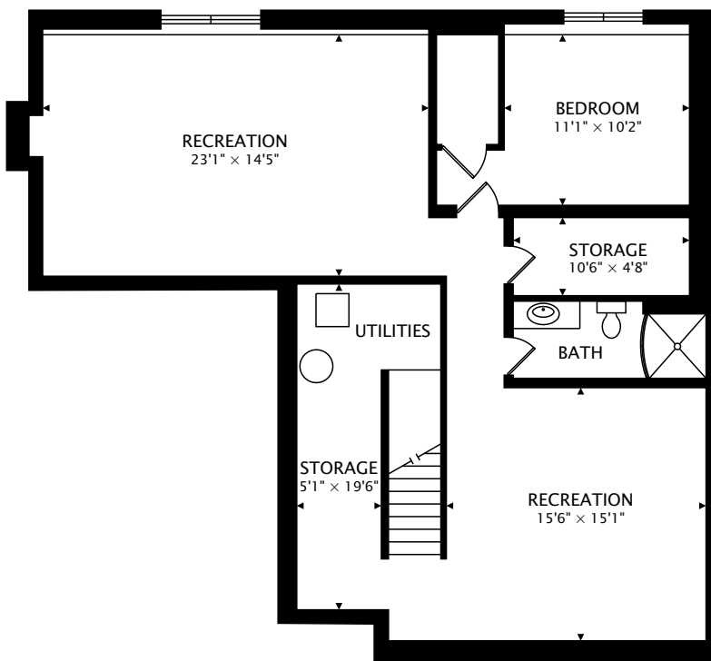
LOWER 1263 sq ft BELOW GRADE
