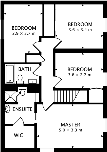
SECOND 90.4 m 2
