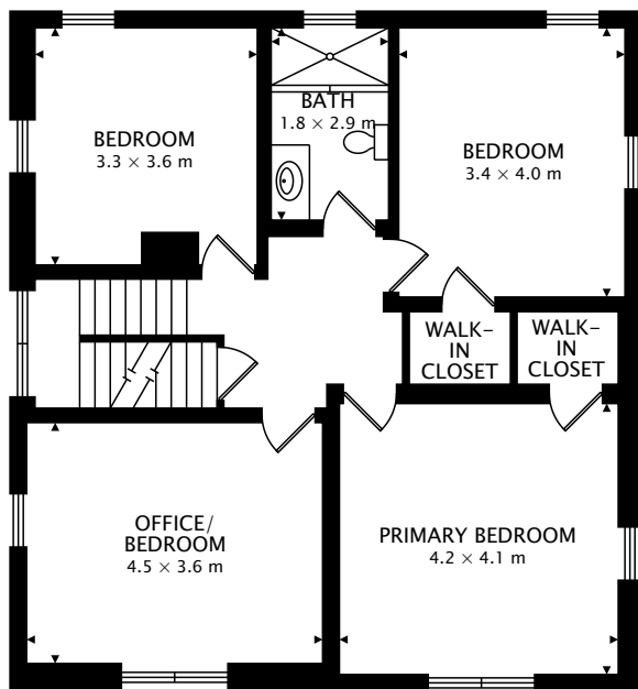
SECOND 91.2 m 2
