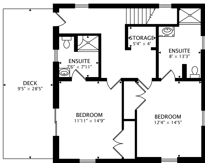
SECOND 836 sq ft
