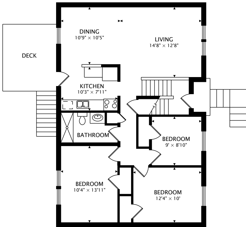
MAIN 1087 sq ft
