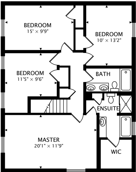
SECOND 1094 sq ft
