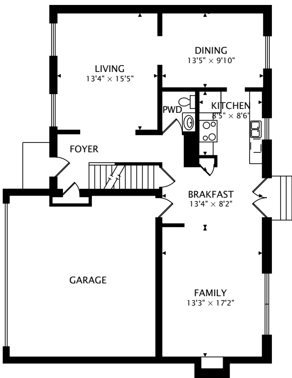
MAIN 1078 sq ft
